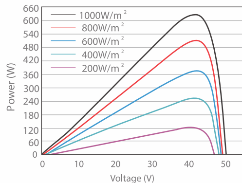
Power-Voltage Curve
